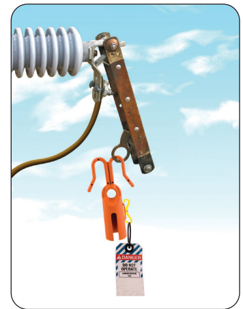
R-TD2 installed on a disconnect switch
