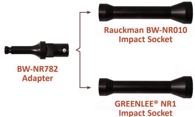
Hex Adapter for 7/16" Quick Change Chuck
